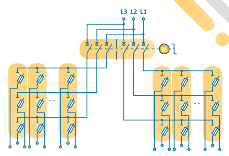
Connection diagram
